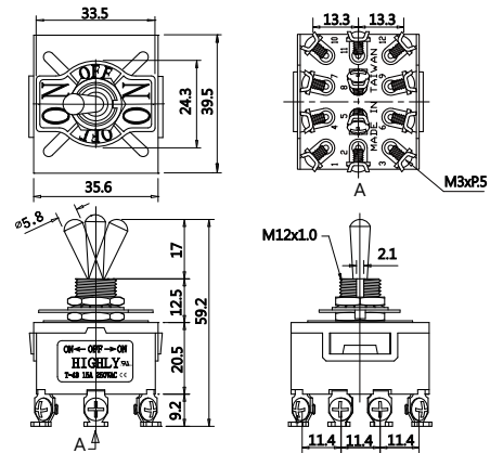
T-42BS / T-43BS 4PDT
