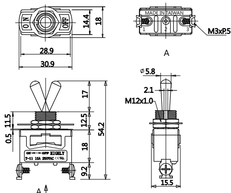
Function Type T-11BS SPST
