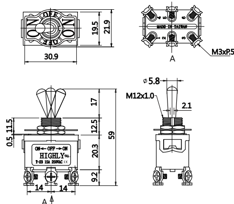
T-22BS / T-23BS DPDT
